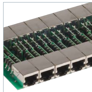
Version with RJ45 sockets shielded on both ends.
