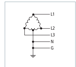
three-phase; 5 conductors Delta "Highleg"
