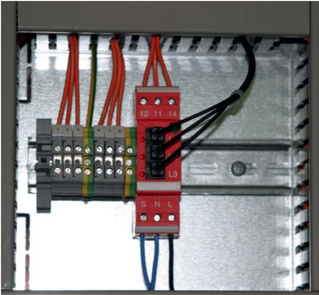
Receiver module for optical transmission with floating changeover contact for DEHNbloc Maxi S and DEHNgap Maxi S surge protective devices.
