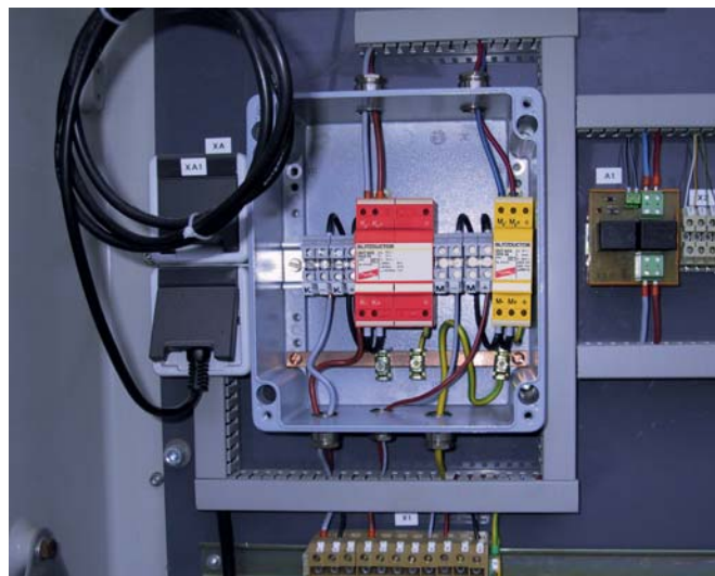
Arrester for protecting active cathodic protection systems. Integrated floating remote signalling contact (break contact) monitors the function of the arrester.
