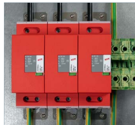
Flexible installation using mounting brackets
