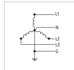
three-phase; 5 conductors
