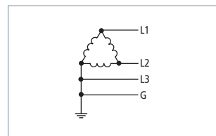
three-phase; 4 conductors Delta "Grounded Corner"
