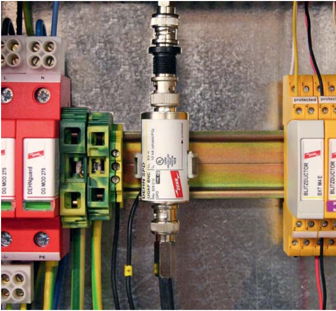
Surge arrester designed as cable adapter for protecting coaxial systems such as video and camera systems from potential damage.
