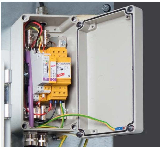
Compact DIN rail mounted surge protective device with screw terminals for multi-core lines.
