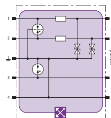
Pluggable SPDs – DIN Rail mounted
