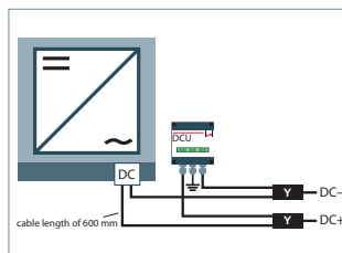
L600 version
