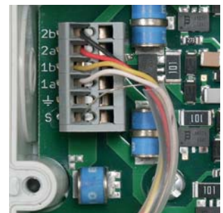
Available with direct or indirect shield earthing (DBX U4/U2 KT BD S 0-180).
