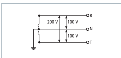
single-phase; 3 conductors (1 Ph, 3 W) 100 V / 200 V
