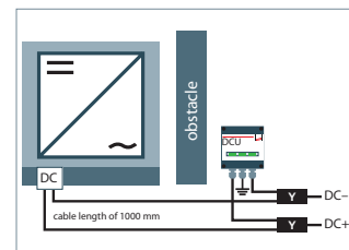
L1000 version
