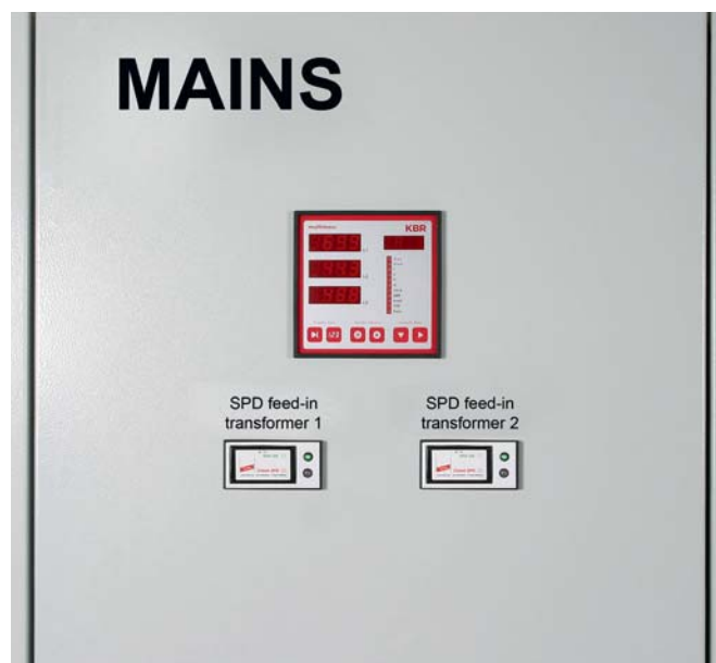
Visual indicator for surge protective devices for installation into switchgear cabinets.
