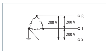
three-phase; 3 conductors (3 Ph, 3 W) 200 V
