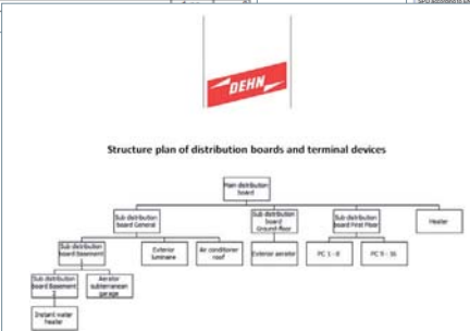
Structure plan
