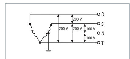
three-phase; + single-phase; 3 conductors + 3 conductors 100 V / 200 V; 200 V
